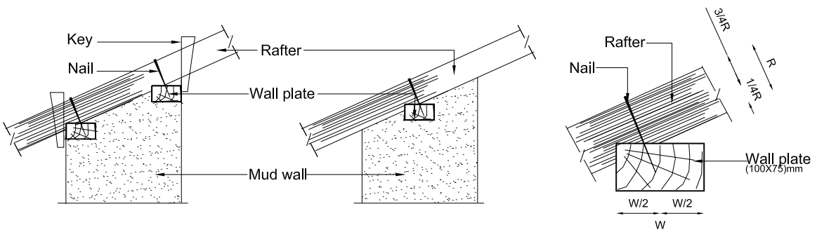
Fixing of rafters to wall plate
