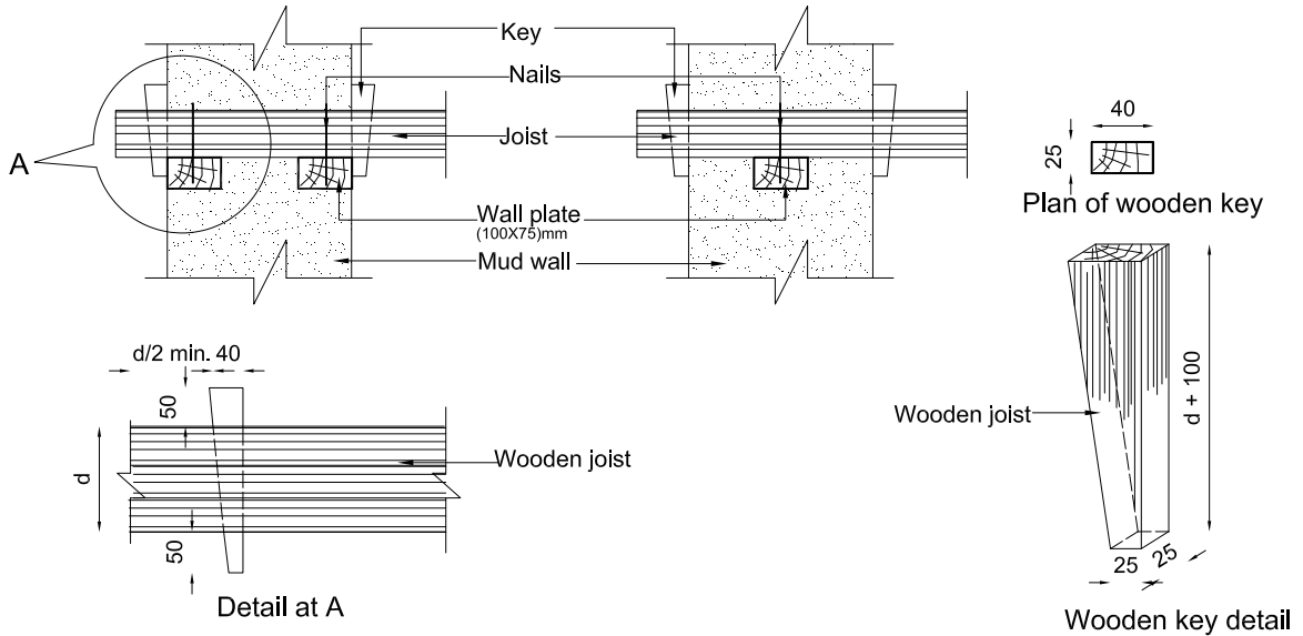
Fixing of joists
