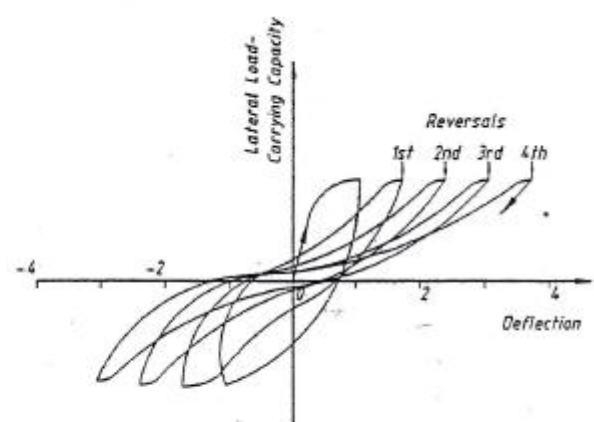
(b) ENERGY DISSIPATION REDUCED WITH EACH REVERSAL
