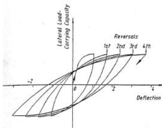
(a) ENERGY DISSIPATION MAINTAINED WITH EACH REVERSAL
