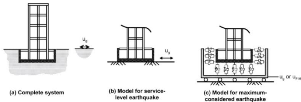
Figure 9-1 Soil-Structure system
