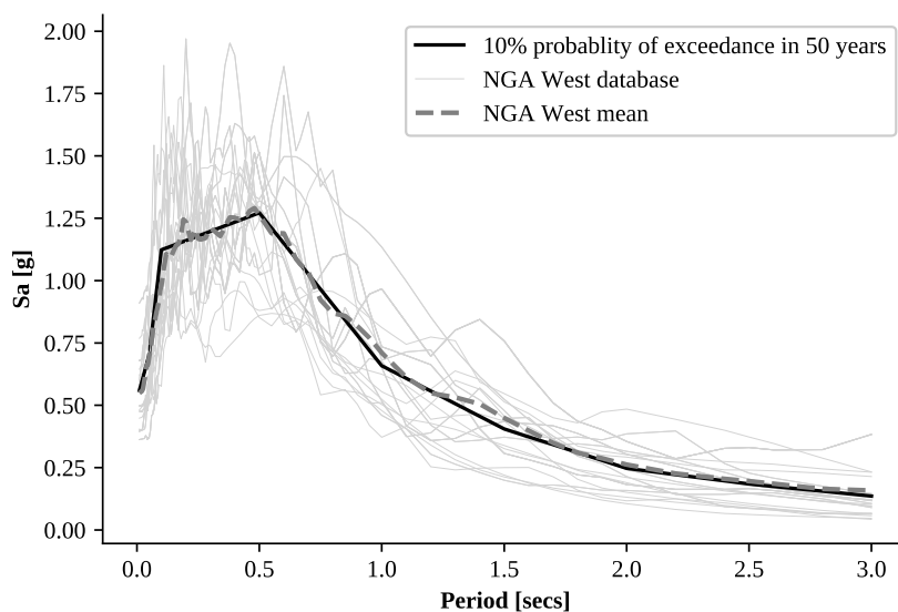
Figure 4-1 Ground motion selection for site response analysis
