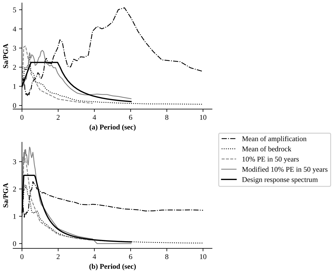
Figure 4-2 Site response results (a) Site D; (b) Site B
