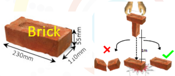
Figure 8: - Brick storage, dimension and method of testing
