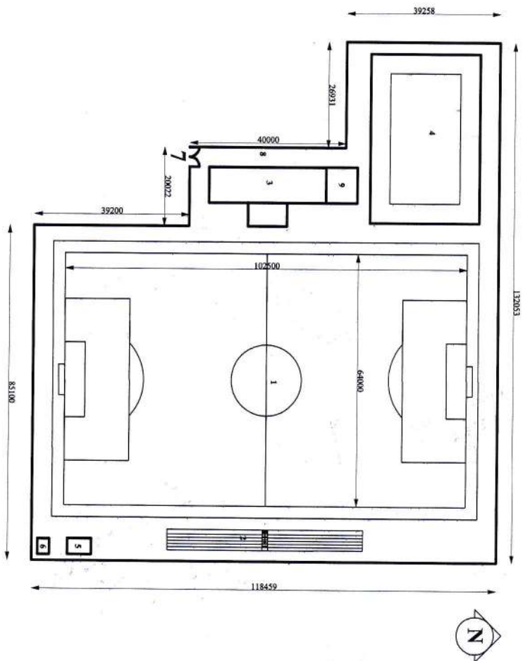
MASTER PLAN OF KHEL GRAM CLUB / RECREATIONAL STANDARD Total land area (25-0-0-0, twenty five ropani , 12725sq.m)
