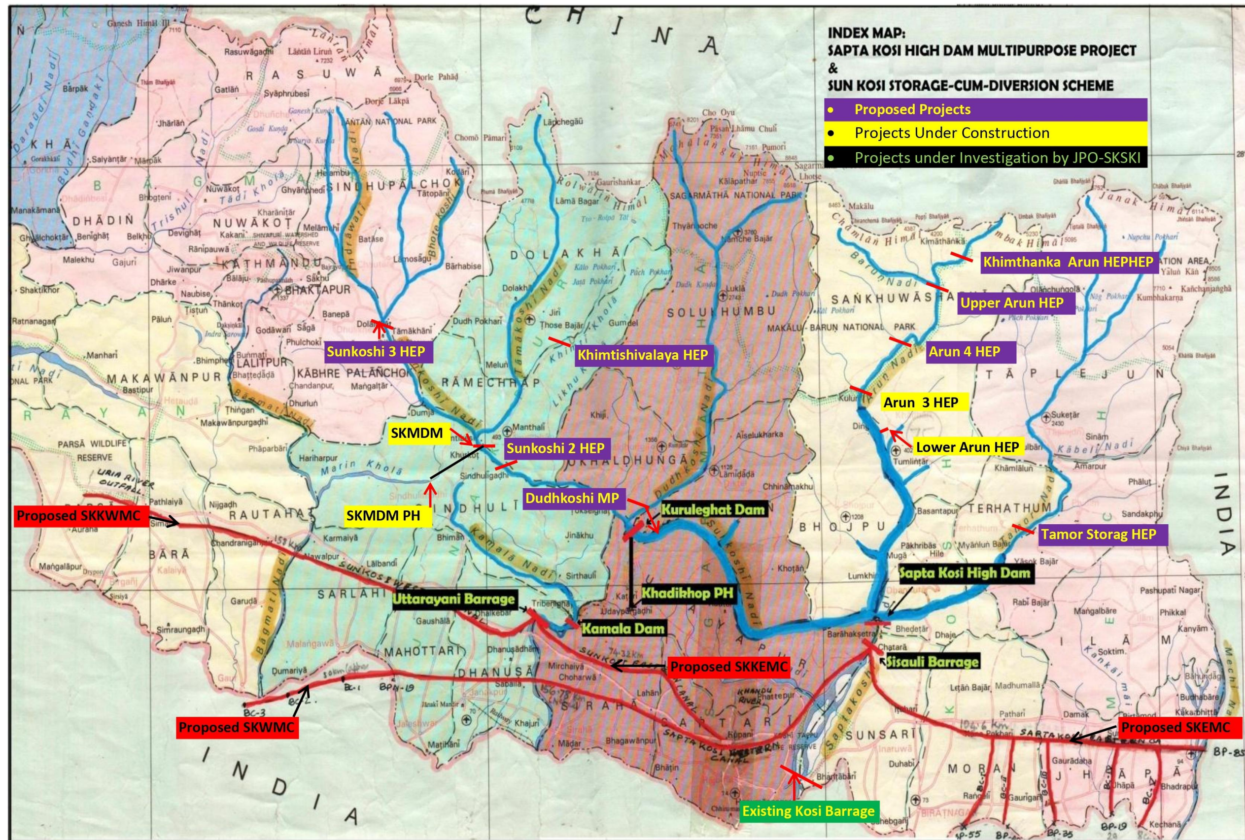
Plate-I: Index Map showing Location of SKSKI Projects
