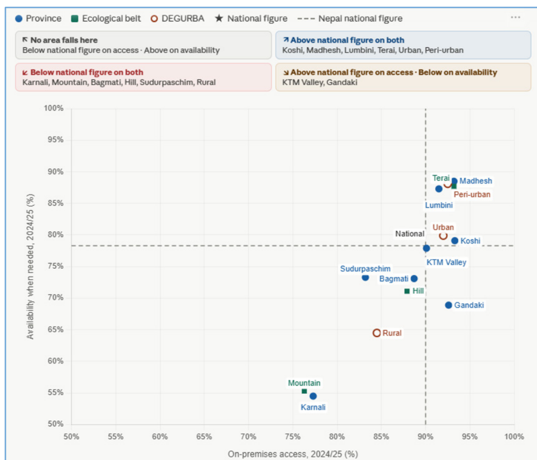
Figure 3.2 Scatterplot 12 of on-premises access versus availability when needed, by province, ecological belt and DEGURBA classification, MICS 2024/25.
