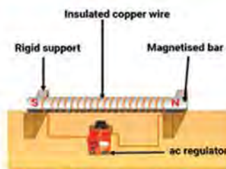
Fig 8.7 Demagnetization by passing alternating current
