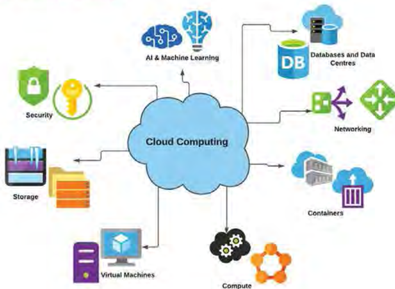
Fig 2.19 Cloud Computing
