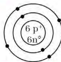
Figure 9.2: Atomic structure
