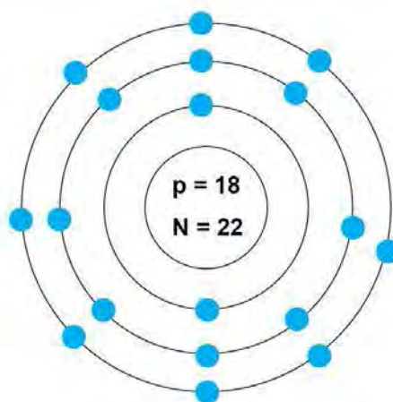
Atom B
