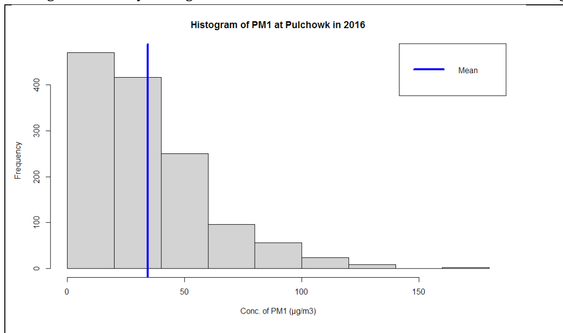
Figure 1. Histogram of PM1 at Pulchowk station in 2016
