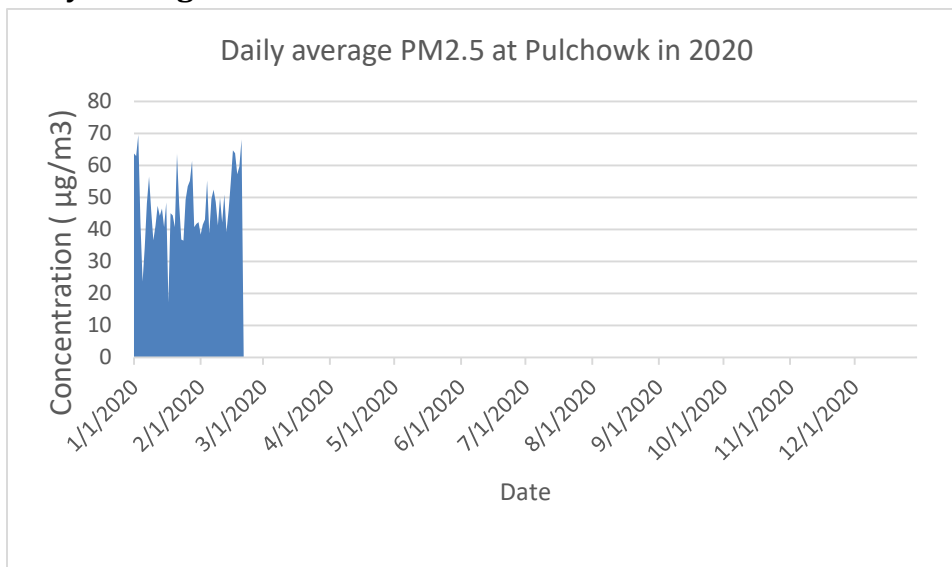
Figure 109. Daily average PM2.5 at Pulchowk station in 2020
