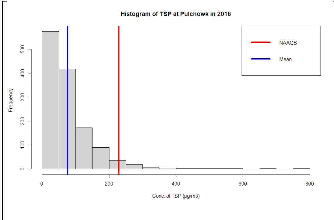
Figure 17. Histogram of TSP at Pulchowk station in 2016
