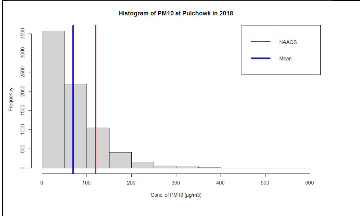
Figure 62. Histogram of PM10 at Pulchowk in 2018
