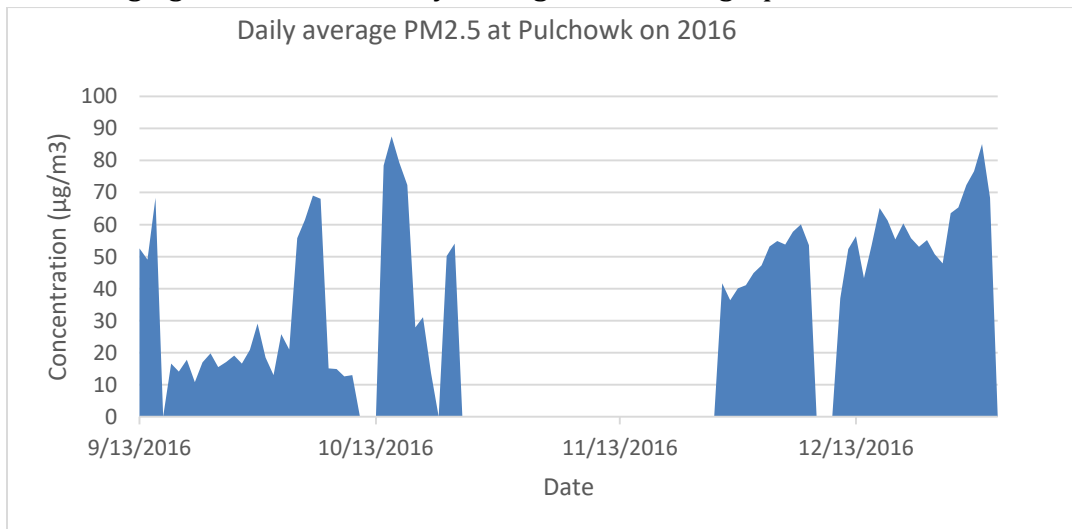
Figure 7. Daily average PM 2.5 at Pulchowk station on 2016
