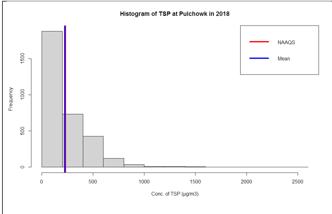
Figure 69. Histogram of TSP at Pulchowk station in 2018
