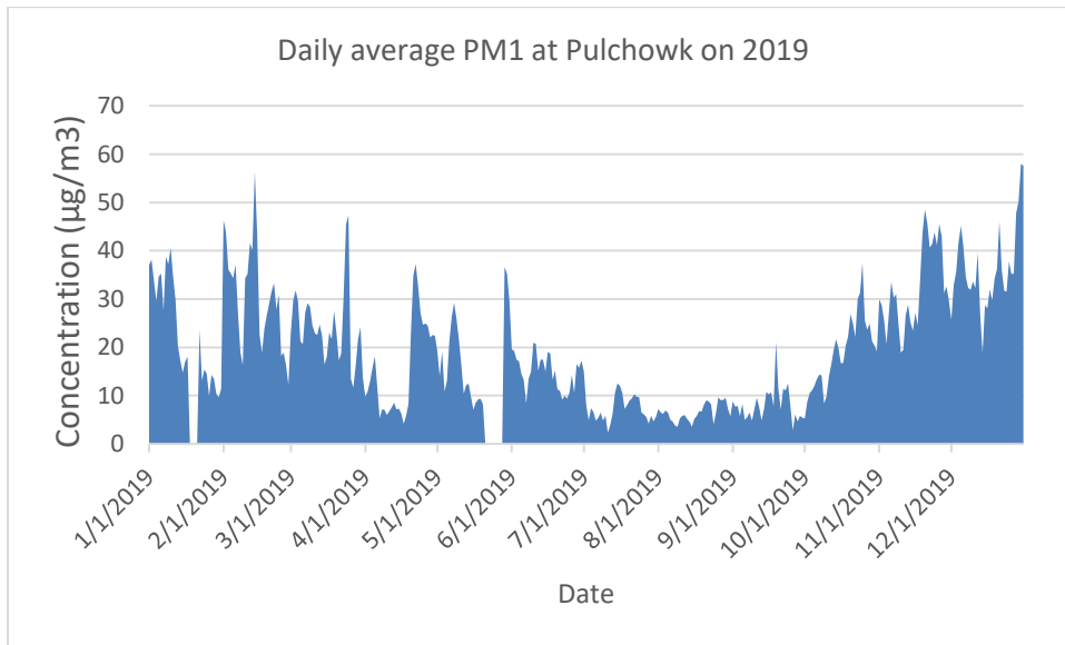
Figure 78. Daily average PM1 at Pulchowk station in 2019
