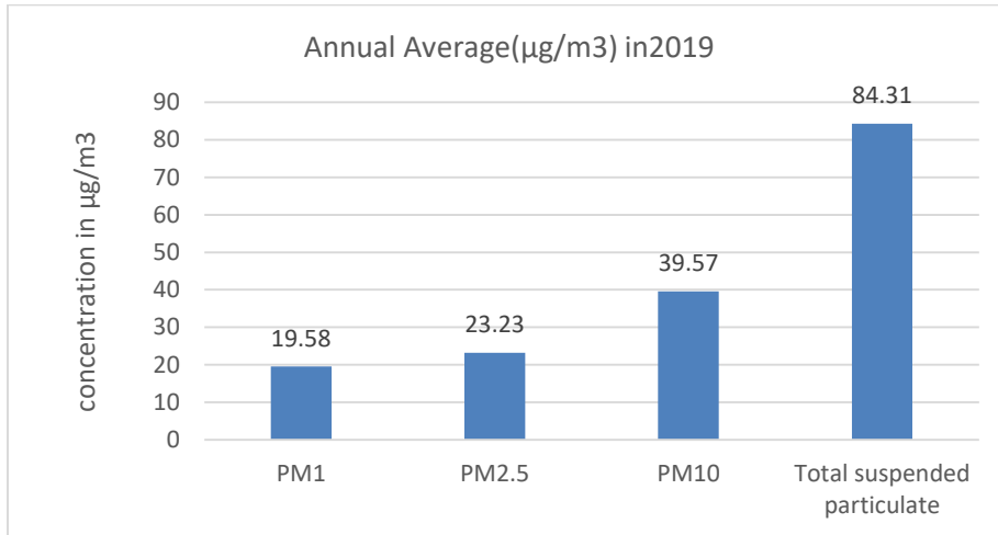
Figure 76. Annual average PM 1 , PM 2.5 , PM 10 and TSp at Pulchowk station for 2019
