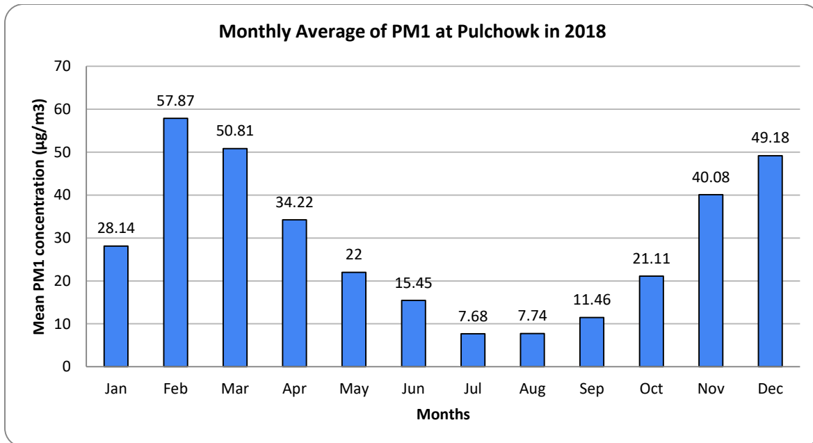
Figure 51. Monthly average PM1 at Pulchowk station in 2018
