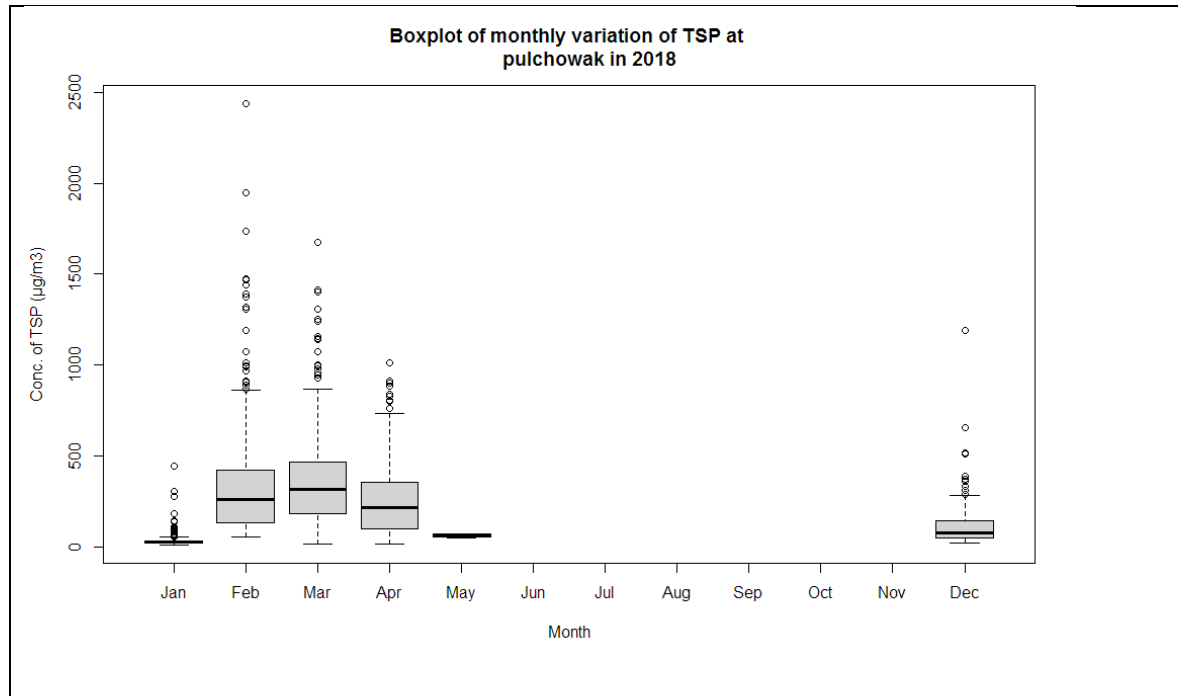
Figure 72. Monthly variation of daily average Total suspended particulate at Pulchowk in 2018
