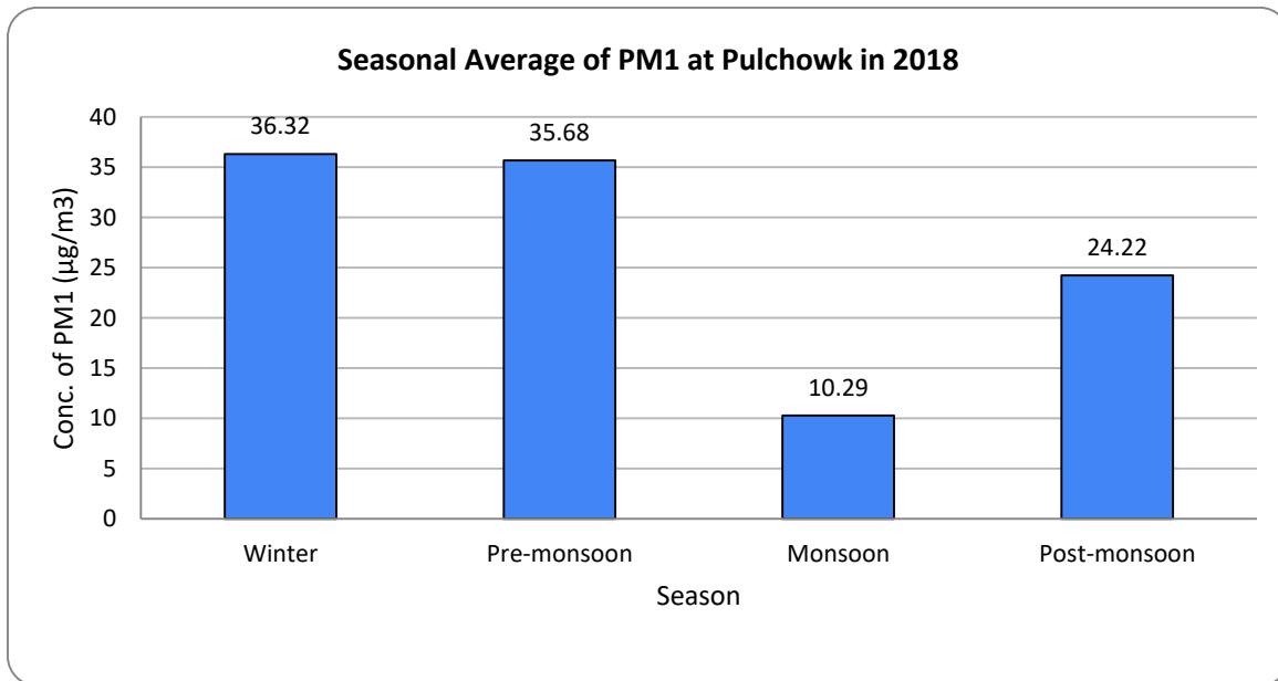
Figure 53. Ambient concentration of average PM1 with four seasons
