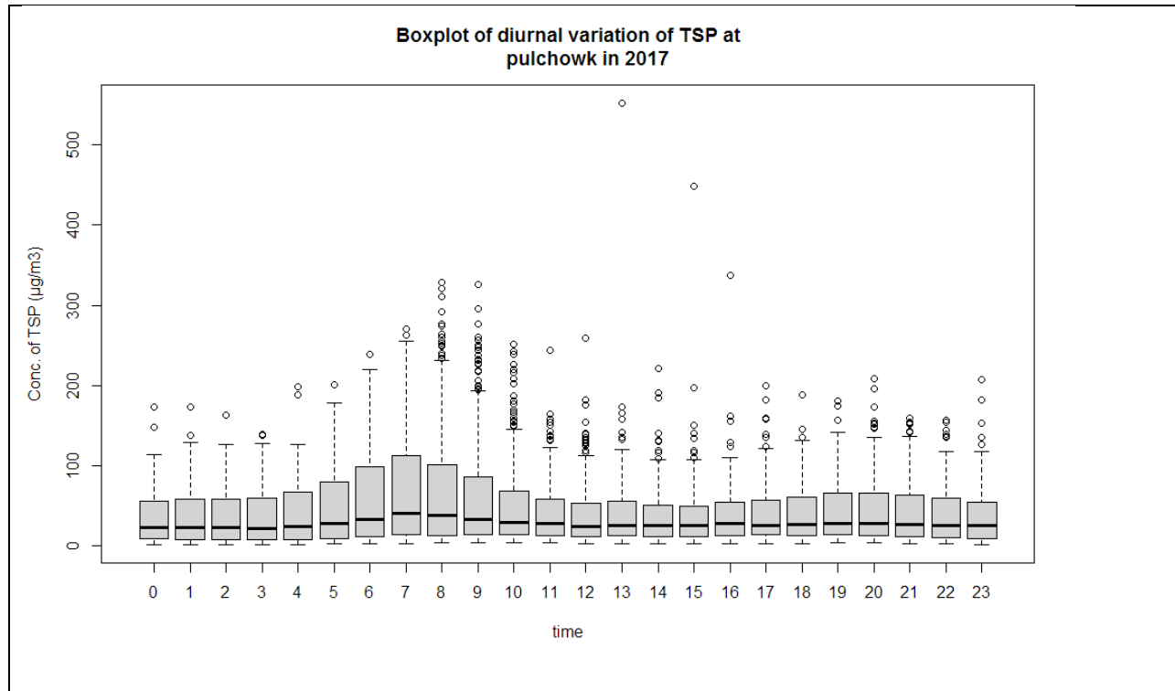
Figure 47. Diurnal variation of TSP at Pulchowk station on 2017
