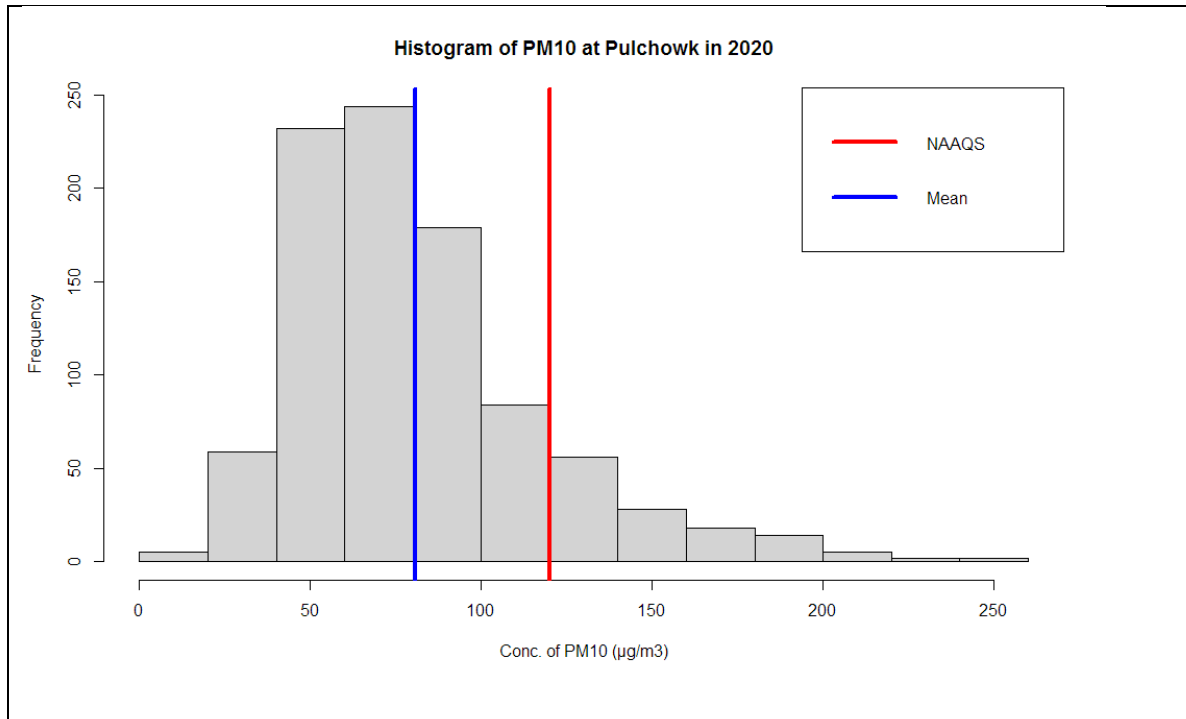
Figure 114. Histogram of PM10 at Pulchowk in 2020
