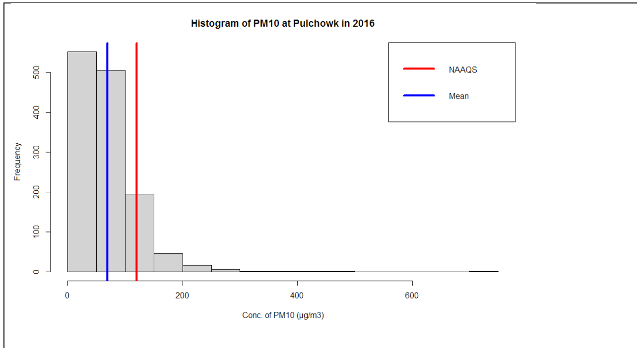
Figure 11. Histogram of PM10 at Pulchowk station in 2016
