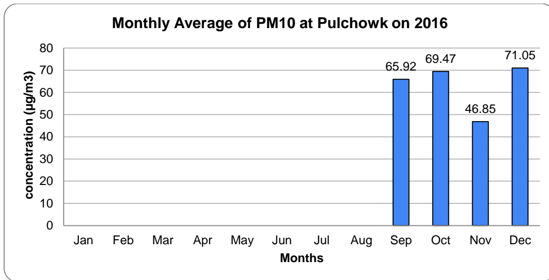
Figure 13. Monthly average PM10 at Pulchowk station in 2016
