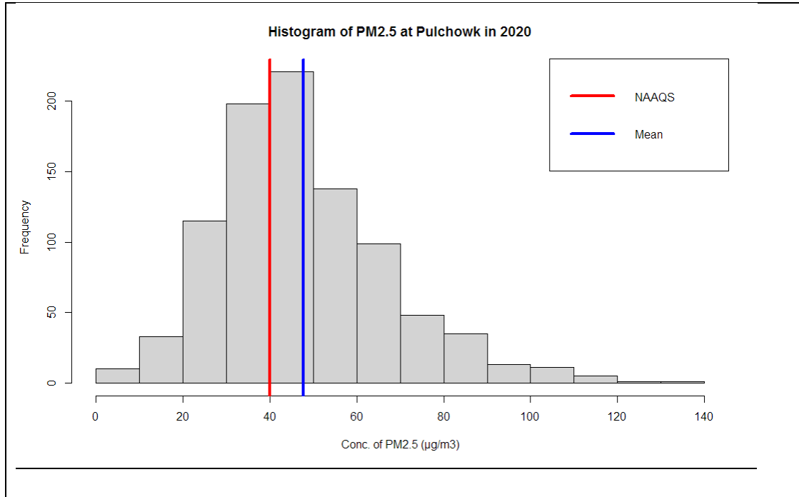
Figure 108. Histogram of PM2.5 at Pulchowk in 2020
