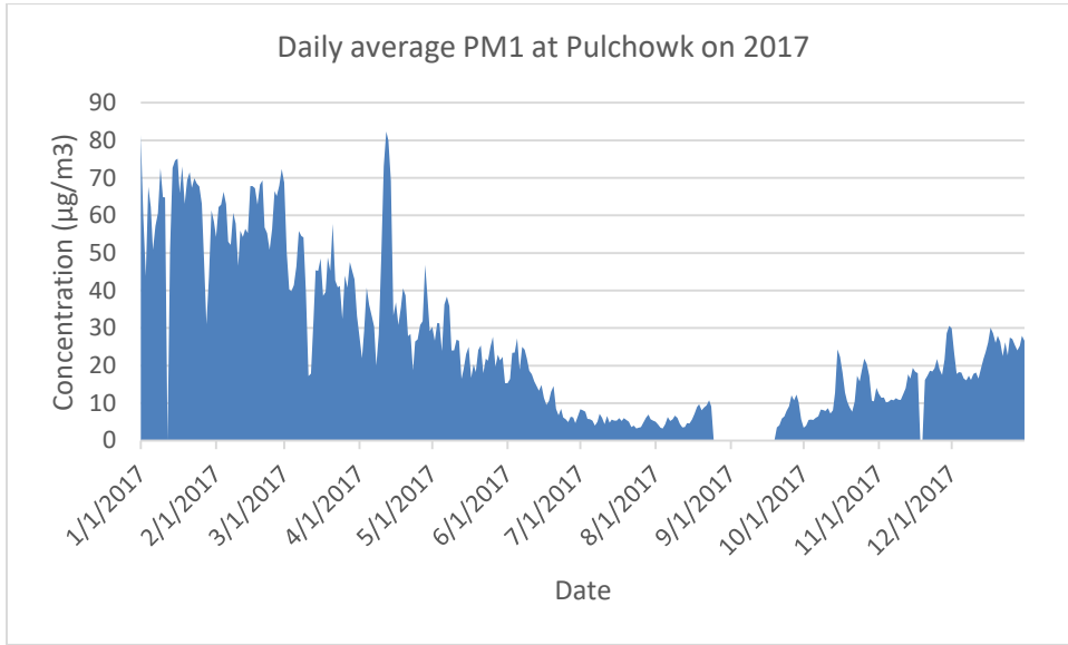
Figure 24. Daily average PM1 at Pulchowk station in 2017
