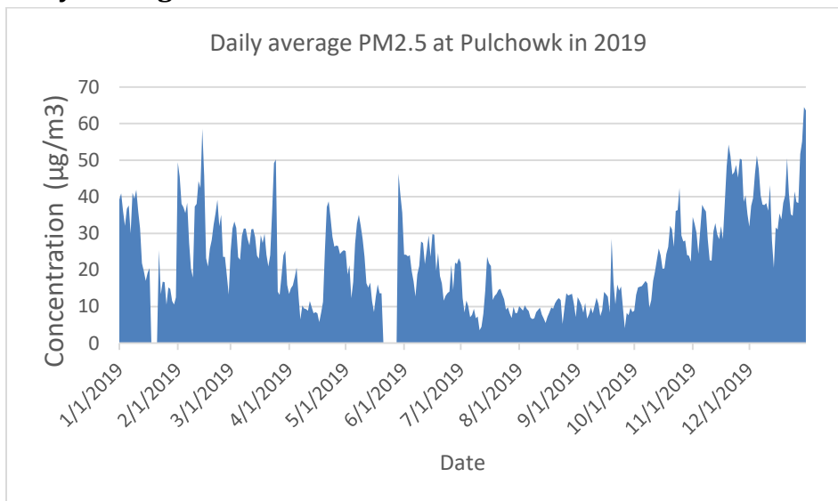
Figure 84. Daily average PM2.5 at Pulchowk station in 2019
