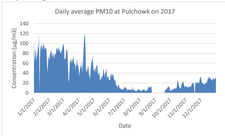
Figure 37. Daily average PM10 at Pulchowk station in 2017
