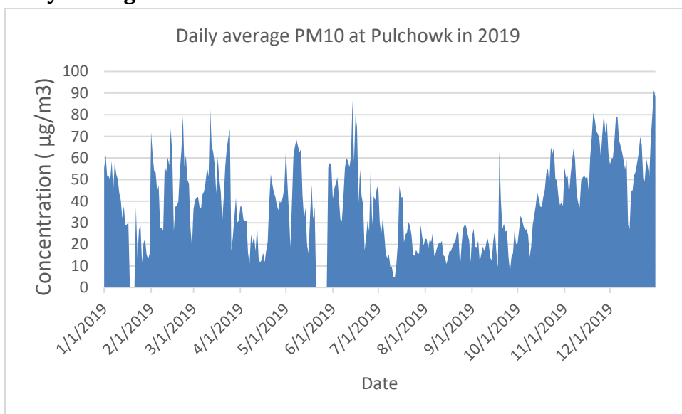
Figure 91. Daily average PM10 at Pulchowk station in 2019
