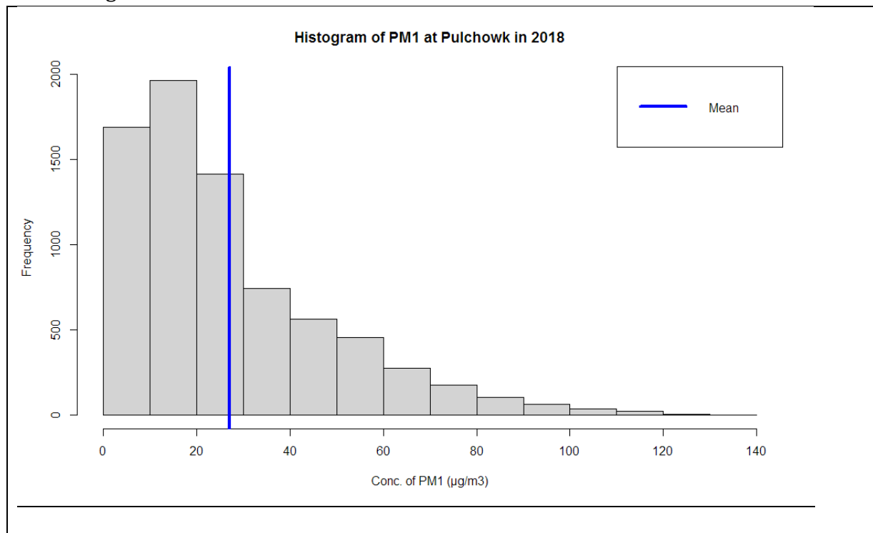
Figure 49. . Histogram of PM1 at Pulchowk in 2018
