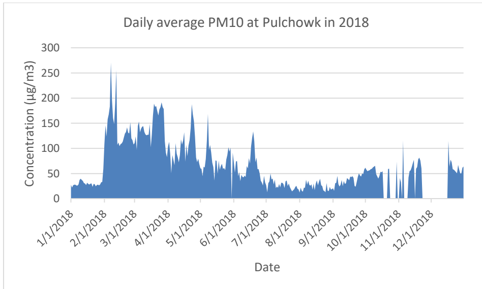
Figure 63. Daily average PM10 at Pulchowk station in 2018
