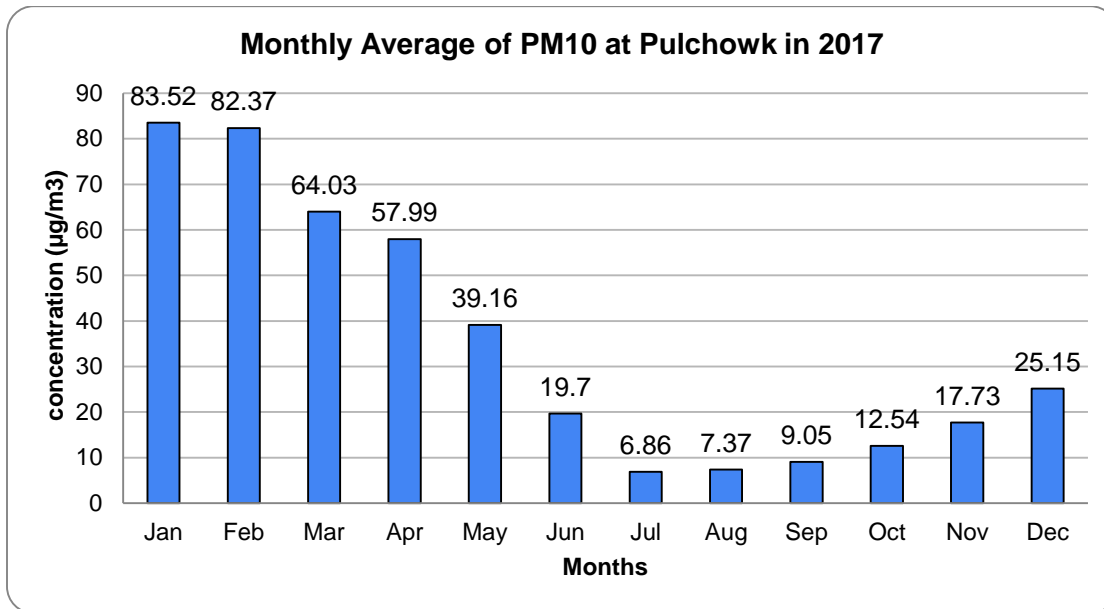
Figure 38. . Monthly average PM10 at Pulchowk station in 2017
