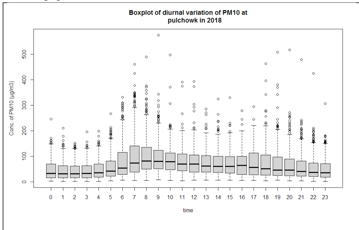
Figure 67. Diurnal variation of Pm10 at Pulchowk in 2018
