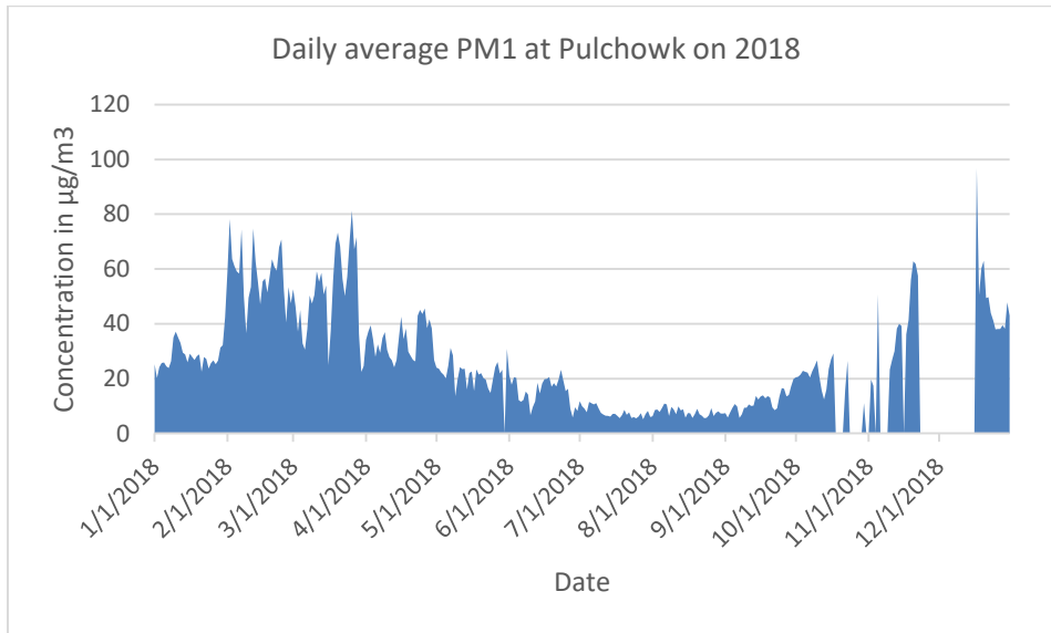
Figure 50. Daily average PM1 at Pulchowk station in 2018
