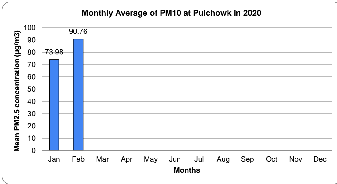
Figure 116. Monthly average PM10 at Pulchowk station in 2020
