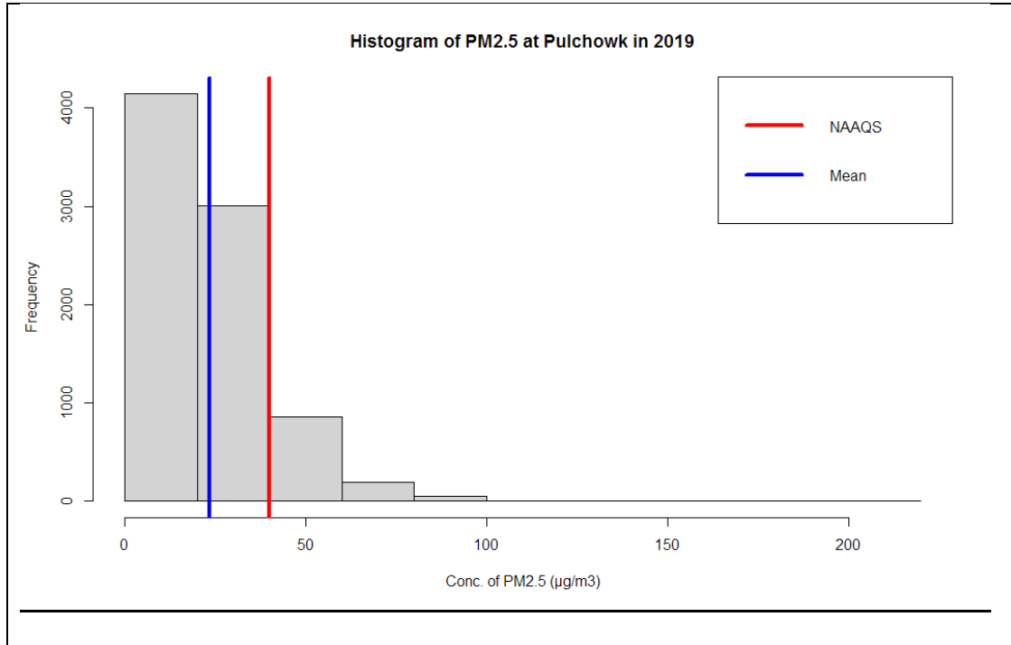
Figure 83. Histogram of PM2.5 at Pulchowk in 2019
