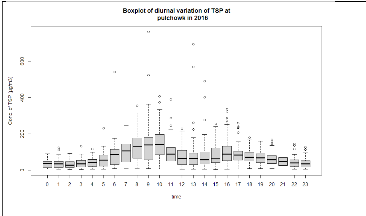
Figure 21. Boxplot of diurnal variation of TSP at Pulchowk in 2016
