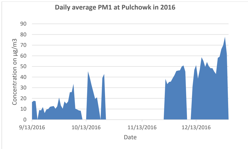
Figure 2. Daily average PM1 at Pulchowk station in 2016
