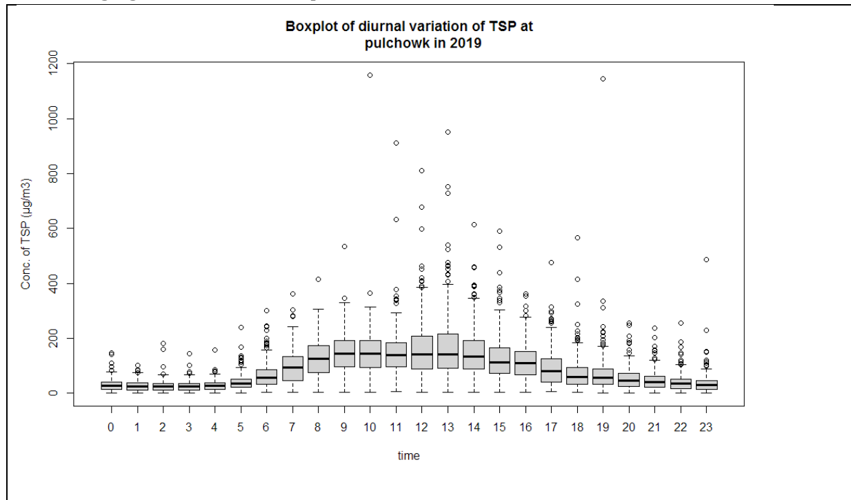
Figure 101. Diurnal variation of TSP at Pulchowk station in 2019
