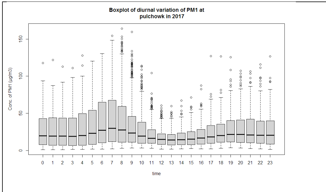
Figure 28. Boxplot of diurnal variation of PM1 at Pulchowk station in 2017
