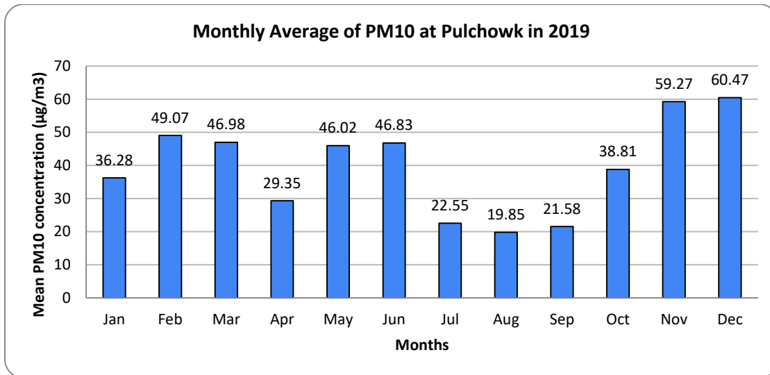
Figure 92. Monthly average PM10 at Pulchowk station in 2019
