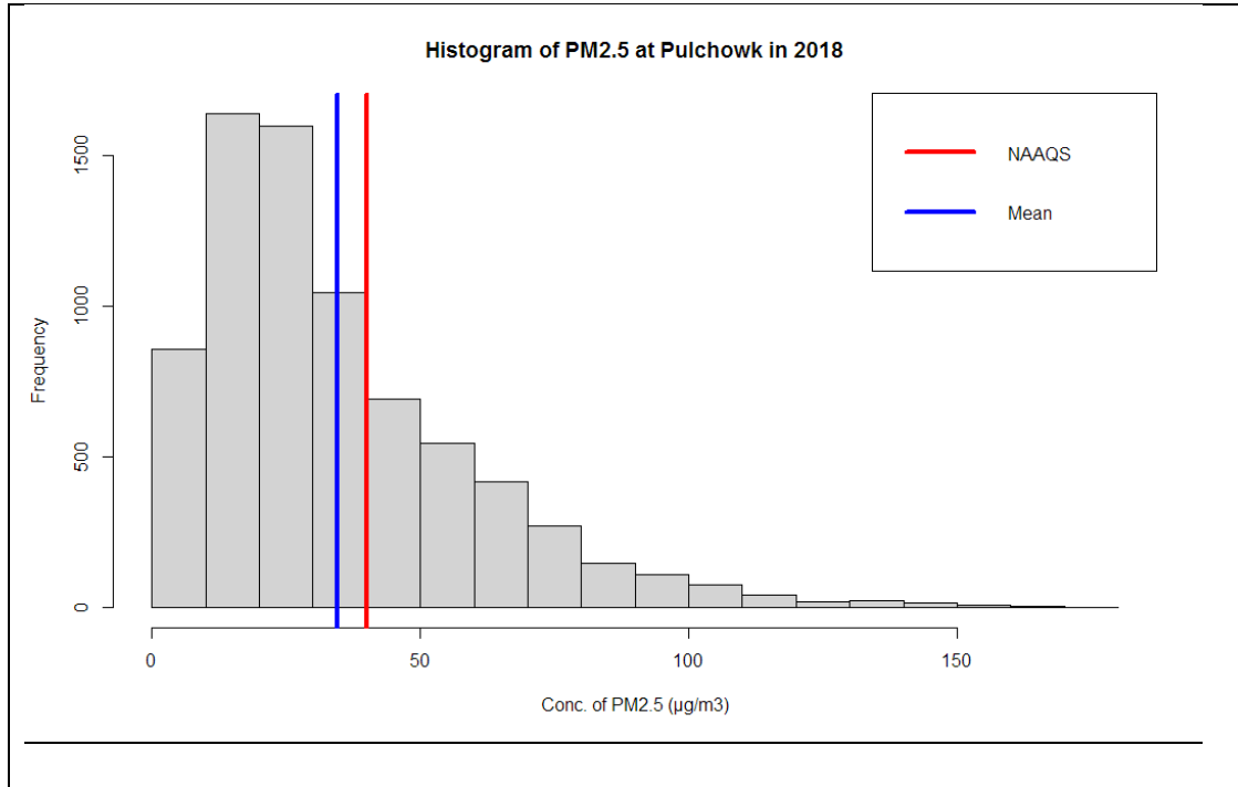
Figure 55. Histogram of PM2.5 at Pulchowk in 2018
