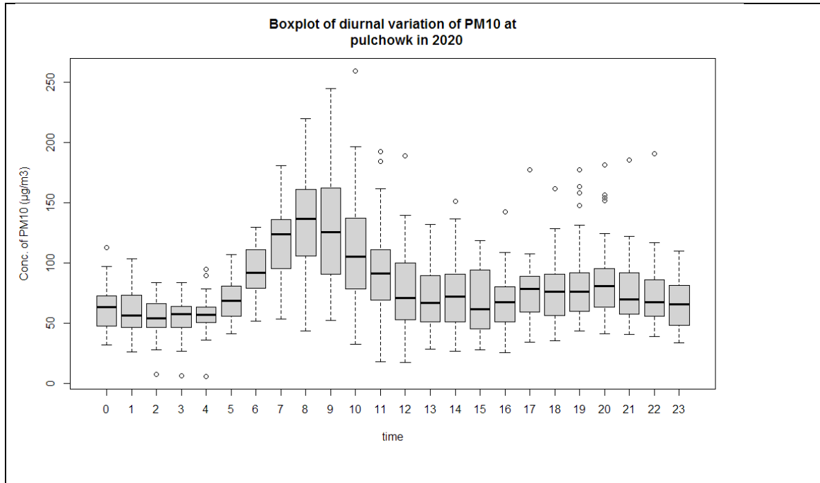
Figure 118. Diurnal variation of Pm10 at Pulchowk in 2020
