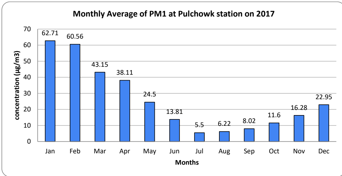
Figure 25. Monthly average PM1 at Pulchowk station in 2017
