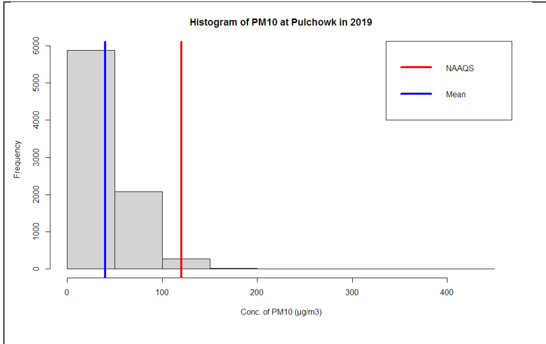
Figure 90. . Histogram of PM10 at Pulchowk in 2019
