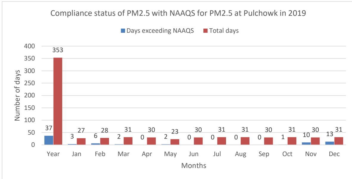
Figure 89. Compliance with National Ambient air quality standard for PM2.5 at Pulchowk station in 2019 Out of total 353 days of Measurement 37 days exceeded the National ambient air quality standard for PM2.5 at Pulchowk station in 2019.
