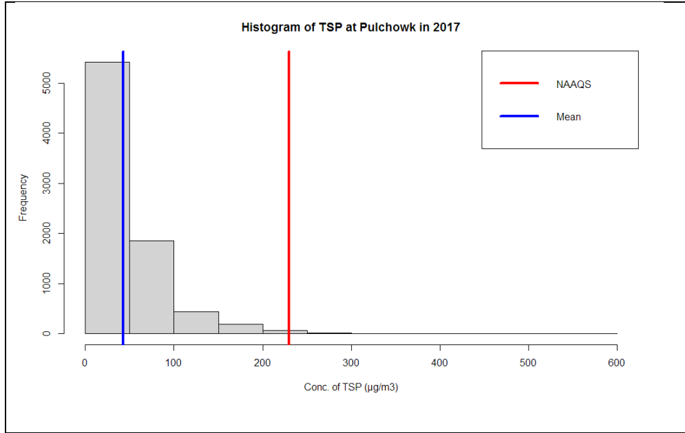
Figure 42. Histogram of TSP at Pulchowk station in 2017
