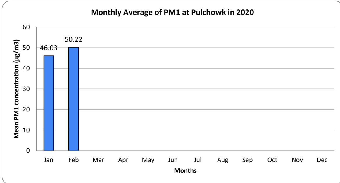
Figure 105. Monthly average PM1 at Pulchowk station in 2020
