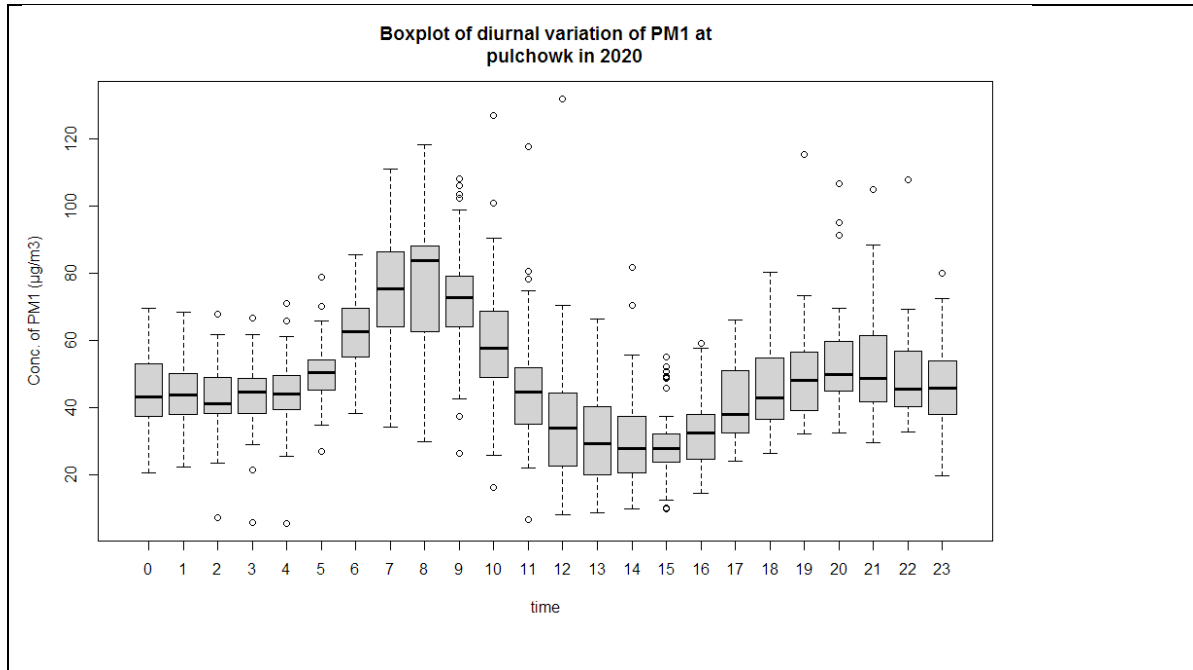
Figure 107. Boxplot of diurnal variation of PM1 at Pulchowk station in 2020
