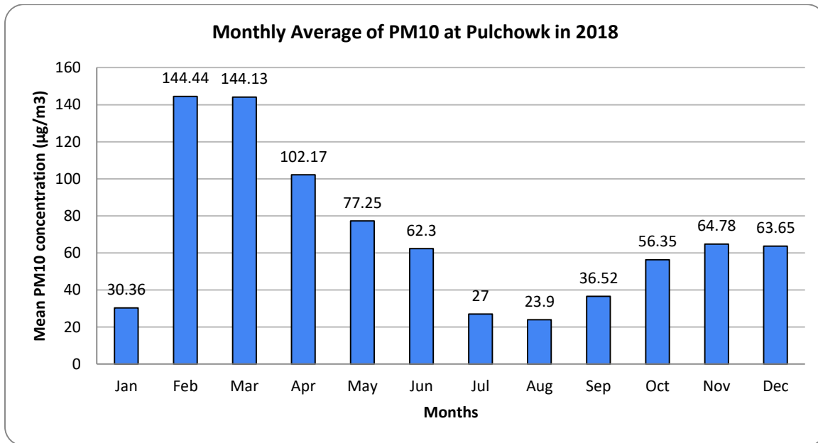
Figure 64. Monthly average PM10 at Pulchowk station in 2018
