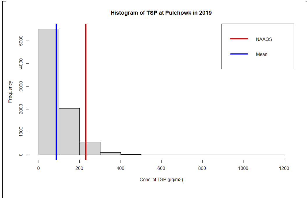
Figure 96. Histogram of TSP at Pulchowk station in 2019
