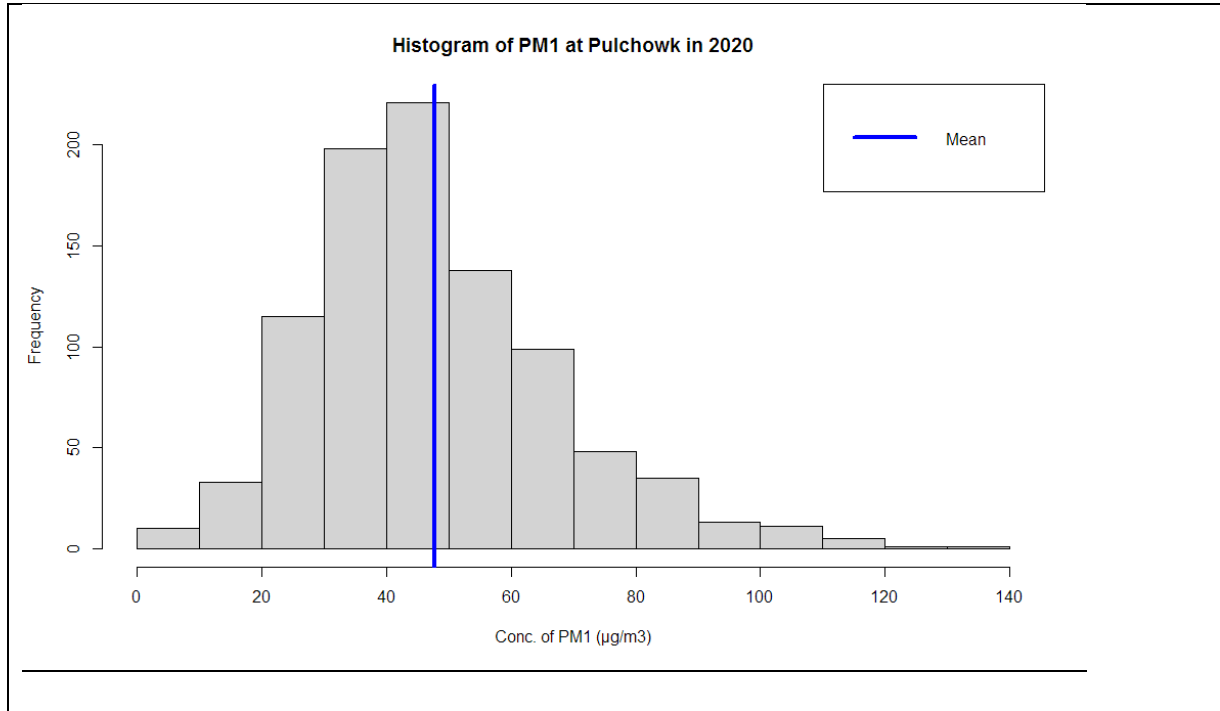
Figure 103. Histogram of PM1 at Pulchowk in 2020
