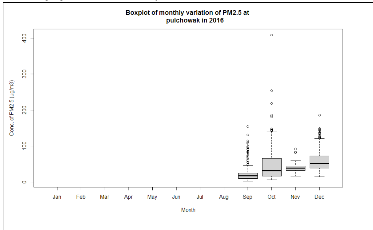
Figure 9. Boxplot of Monthly variation of PM 2.5 at Pulchowk station in 2016
