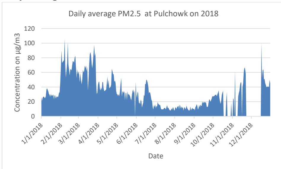
Figure 56. Daily average PM2.5 at Pulchowk station in 2018
