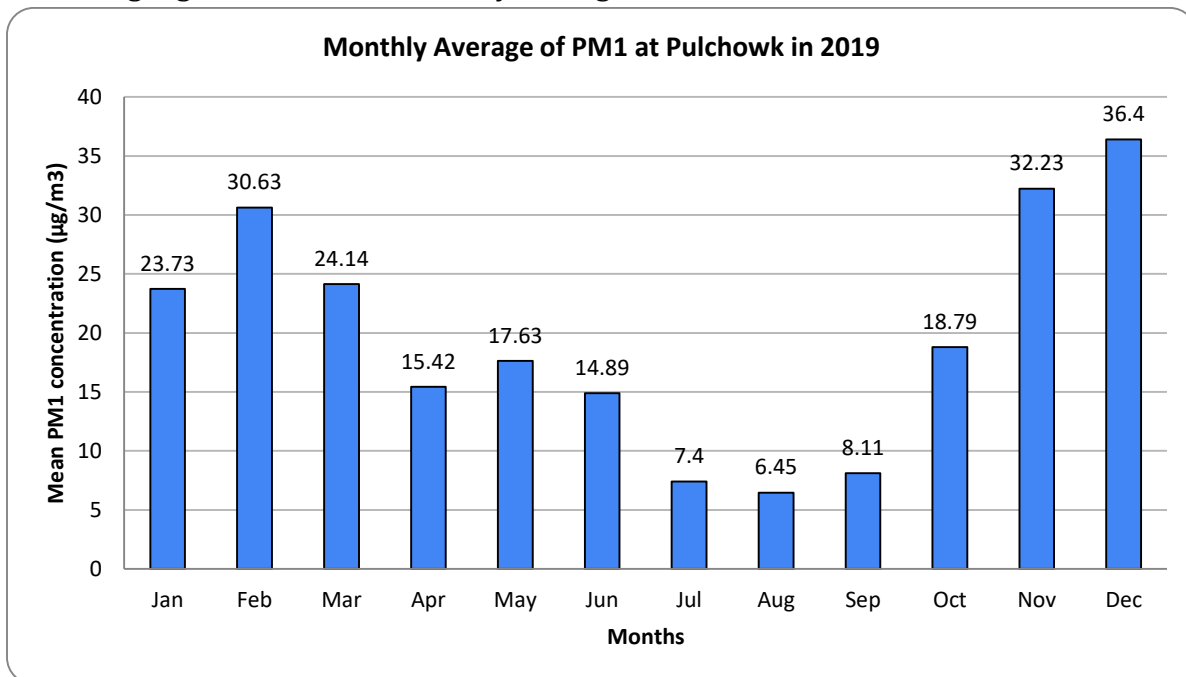
Figure 79. . Monthly average PM1 at Pulchowk station in 2019
