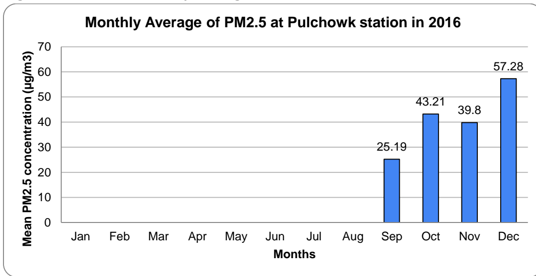
Figure 8. Monthly average PM 2.5 at Pulchowk station in 2016
