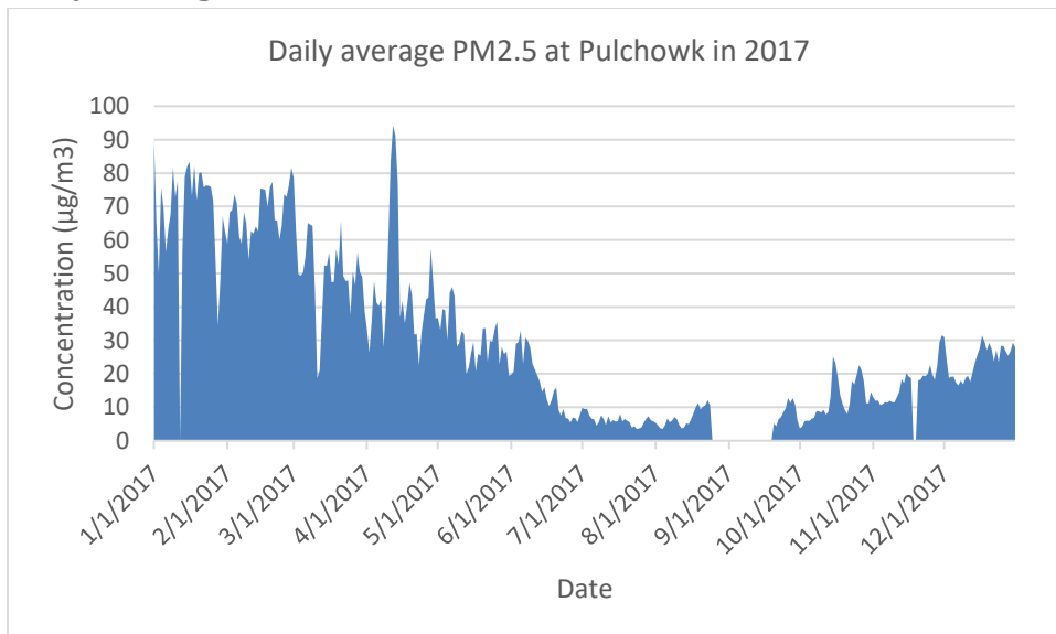
Figure 30. Daily average PM2.5 at Pulchowk station in 2017
