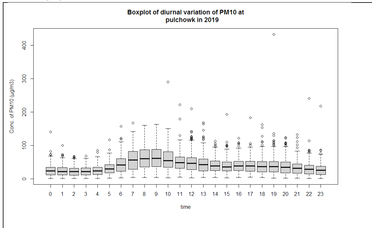
Figure 95. Diurnal variation of Pm10 at Pulchowk in 2019
