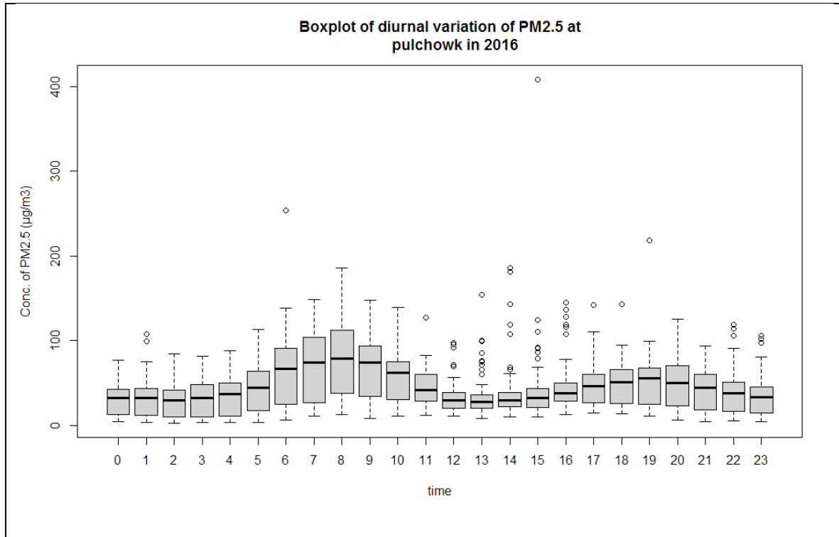
Figure 10. Boxplot of PM2.5 at Pulchowk station in 2016
