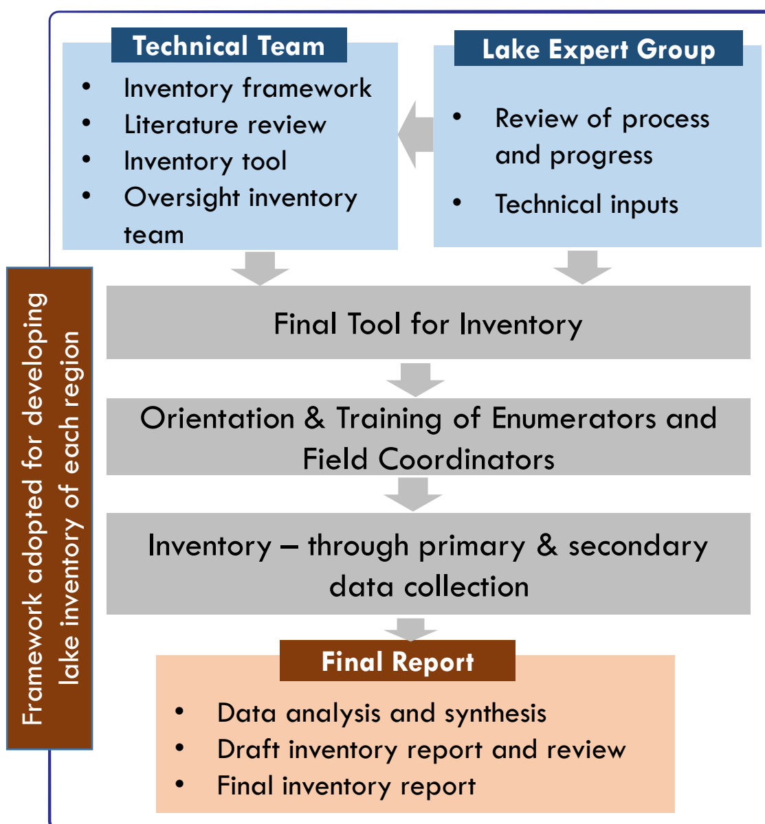
Figure 3-1 | Methodological framework for inventory of Himalayan lakes in Nepal
