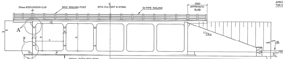
ELEVATION OF BOX CULVERT : HALF AT SECTION 2-2 , HALF AT VIEW 3-3
