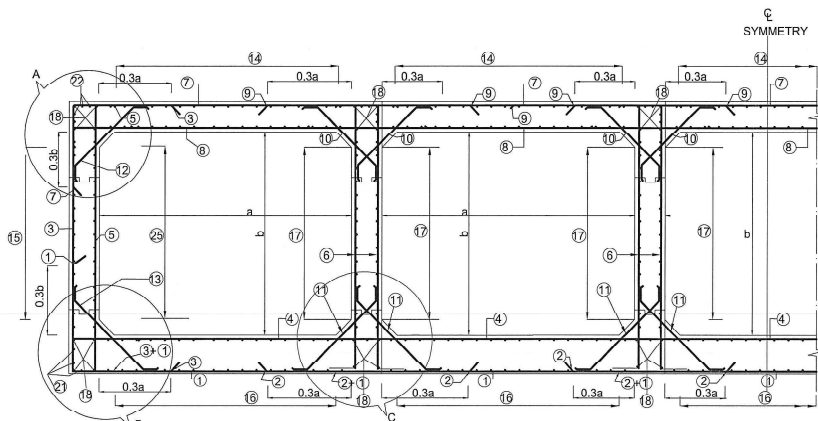
REINFORCEMENT DETAILS OF FIVE CELL BOX CULVERT
