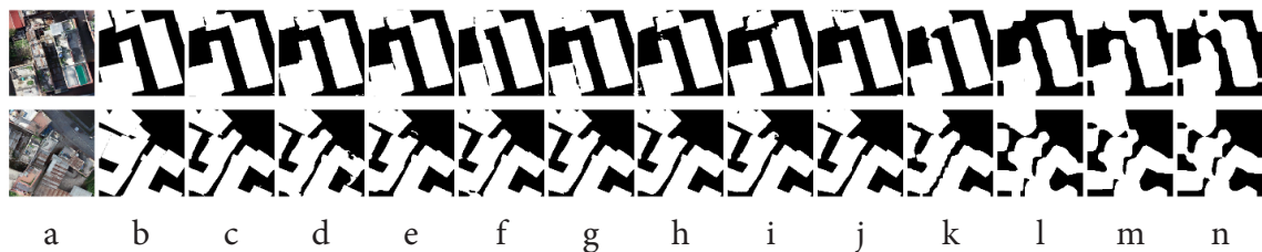
Figure 7: Performance comparison on the custom dataset with Model trained in Massachusetts. (a) Original Image, (b) Ground Truth (c) Linknet-Vgg19, (d) Linknet-resnet18, (e) Linknet-resnet34, (f) Linknet-resnet50, (g) Unet-Vgg19, (h) Unet-resnet18, (i) Unet-resnet34, (j) Unet-resnet50, (k) PSPNet-Vgg19, (l) PSPNet-resnet18, (m) PSPNet-resnet34, and (n) PSPNet-resnet50
