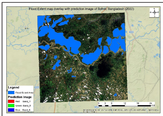
Figure 6: Predicted Flooded areas of Sylhet, Bangladesh
