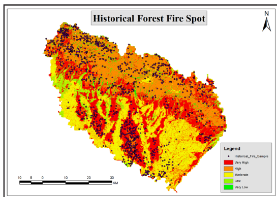
Figure 6 Spatial distribution of historical fire spots
