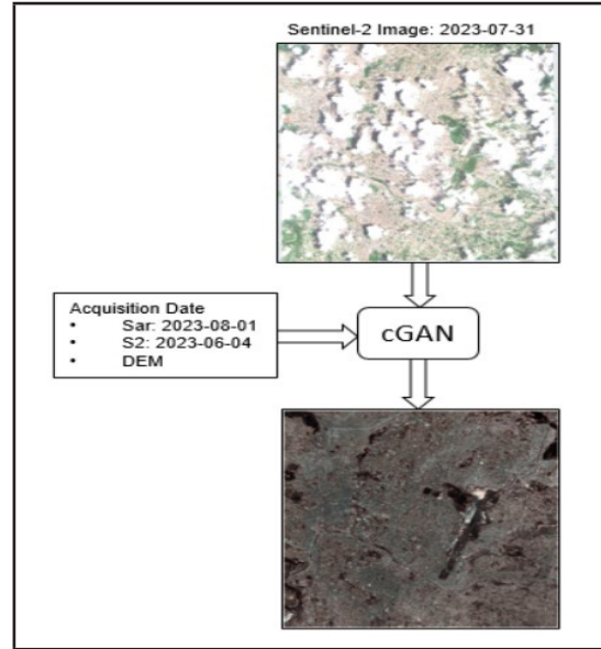
Figure 6: A_cGAN_SOD outcome
