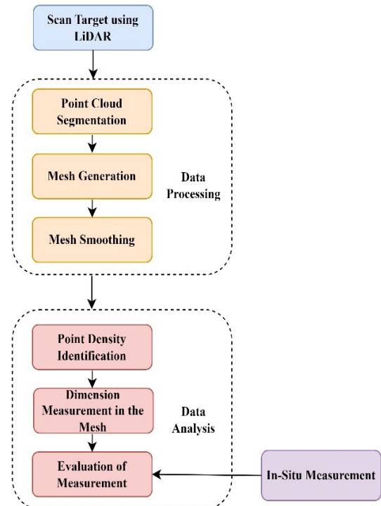
Figure 2: Methodological flowchart
