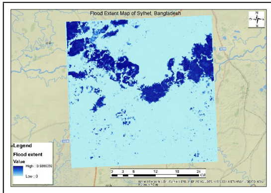
Figure 5: Flood extent map
