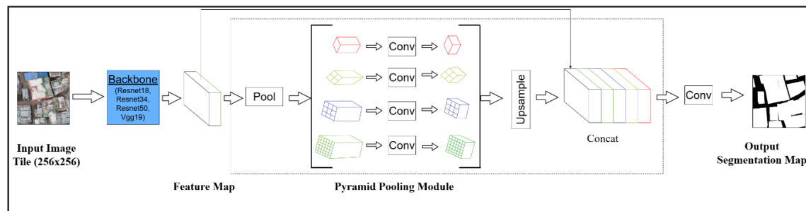
Figure 5: PSPNet Architecture
