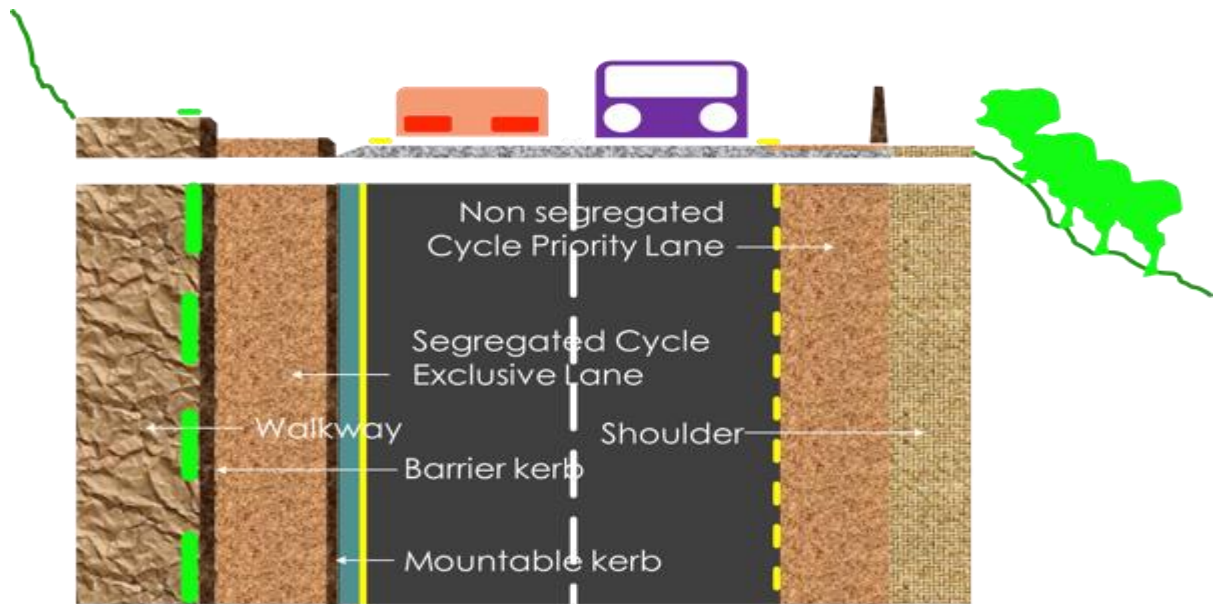
Figure 22: Typical Drawing of Main Road (Source: Nepal Urban Roads Standard 2071)
