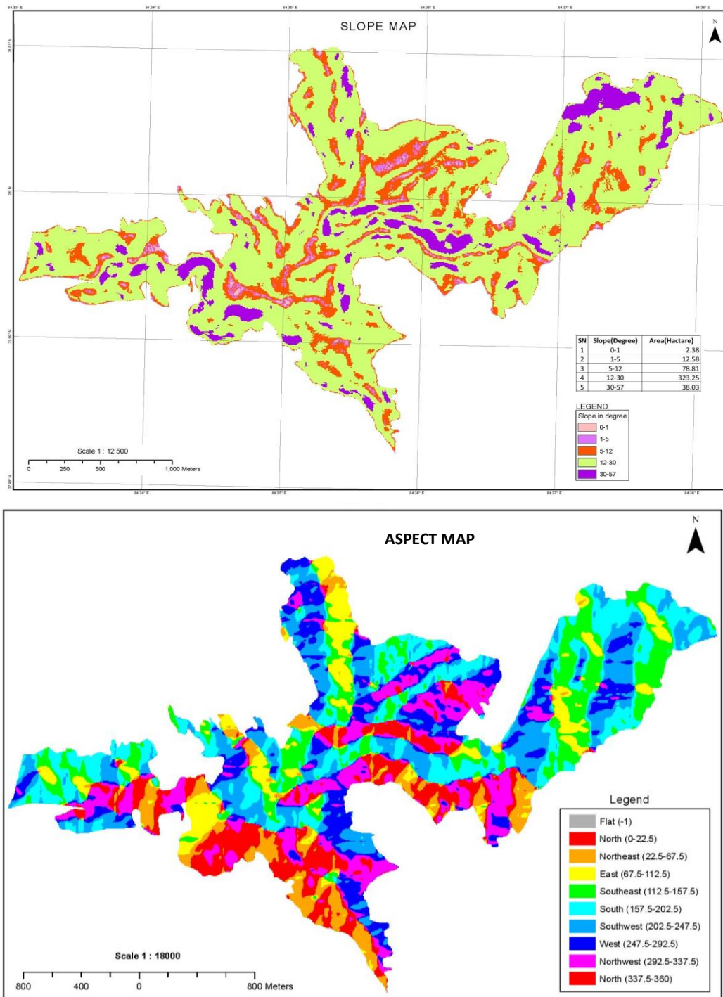
Figure 7: Slope and Aspect Map
