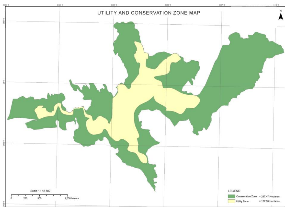
Figure 15: Utility and Conservation zone
