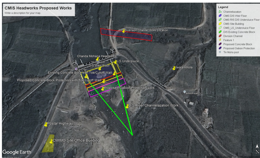
Project Location and proposed work map
